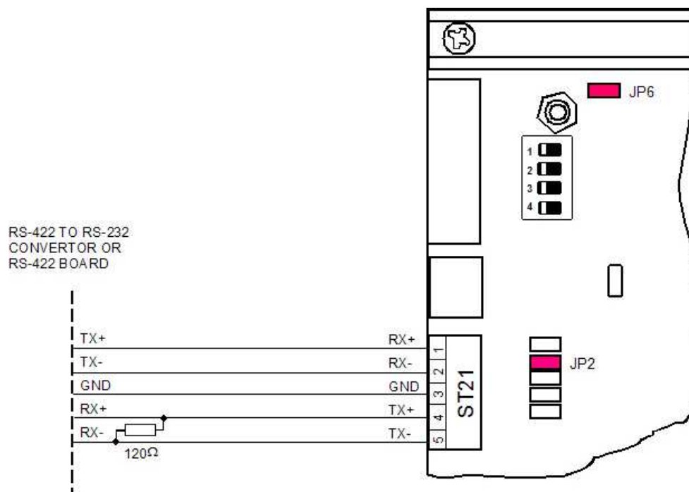
Figure 2-11. RS-422 Interface Connection
