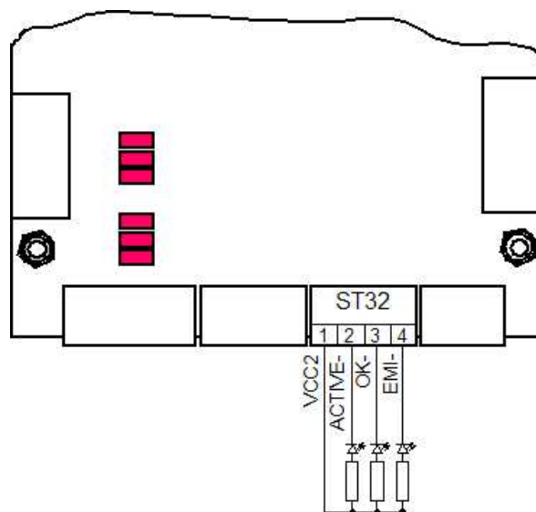
Figure 2-19. Indicator Outputs
